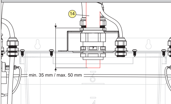
Detail 15.1
